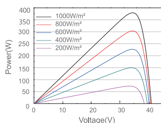
Power-Voltage Curve JAM60S20-380/MR/1000V
